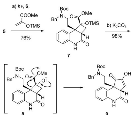
Scheme 2. Synthesis of the tricyclic intermediate 9 by a sequence of enantioselective [2+2] photocycloaddition and rearrangement: a) h\nu (370 nm), 6 (2.5 equiv), silyl enol ether (5.0 equiv), toluene, -60^{\circ}\text{C} , 4 h, 76%; b) \text{K}_2\text{CO}_3 , MeOH, 20^{\circ}\text{C} , 2 h, 98%.
