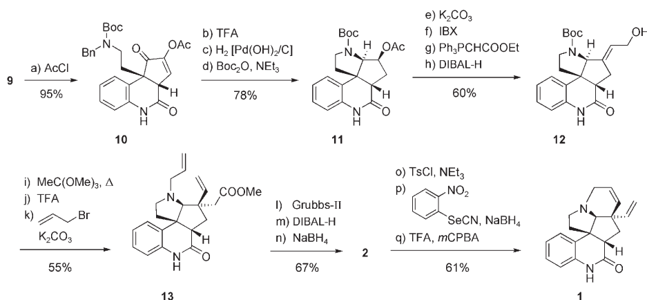
Scheme 3. Completion of the total synthesis of (+)-meloscine ( 1 ) starting from tricyclic ketone 9 :
