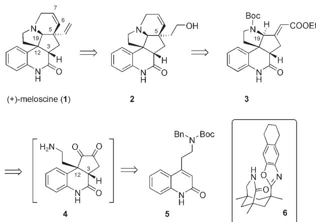
Scheme 1. Retrosynthetic analysis of (+)-meloscine. Boc = tert -butoxycarbonyl, Bn = benzyl.
